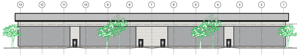
West Elevation .
